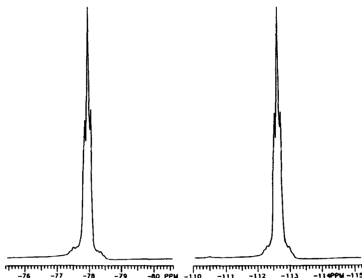
FIGURE 5 ^{19}\text{F} NMR spectra of [(\text{TTBP})\text{SiF}_4][\text{K-18-crown-6}] in \text{CD}_2\text{Cl}_2 at -73^\circ\text{C} . \delta(^{19}\text{F}_{\text{ak}}) = -77.98 ppm; J_{\text{SiF}} = 248 Hz; \delta(^{19}\text{F}_{\text{eq}}) = -112.7 ppm; J_{\text{SiF}} = 191 Hz; J_{\text{F-Fit}} = 29.6 Hz.
