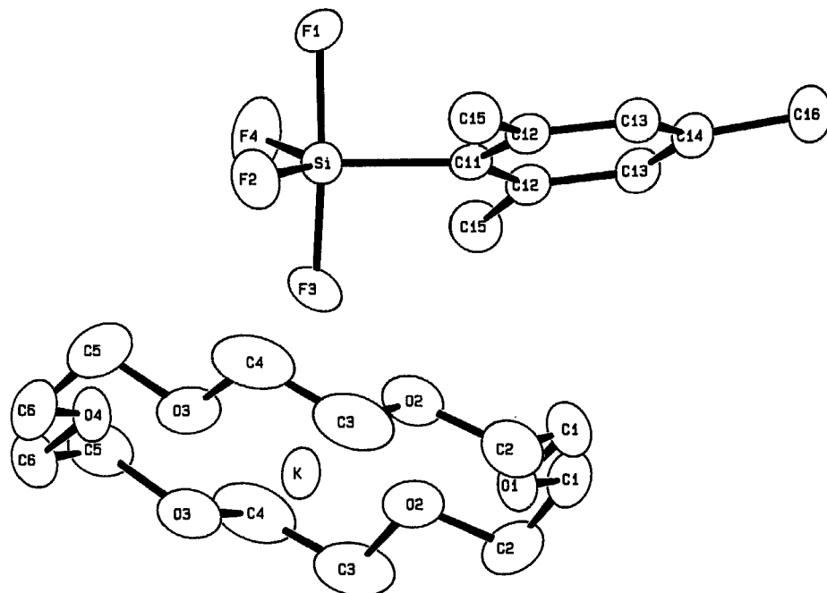
FIGURE 2 ORTEP plot of [\text{Me}_3\text{C}_6\text{H}_2\text{SiF}_4][\text{K-18-crown-6}] (2) with thermal ellipsoids at the 30% probability level. Atoms with the same labels are related by a crystallographic mirror plane ( x, \frac{1}{2} - y, z ). For purposes of clarity, only one set of positions is shown for the fluorine atoms and hydrogen atoms are omitted.
