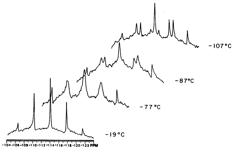
FIGURE 4 Variable-temperature ^{29}\text{Si} NMR spectra of [(\text{TTBP})\text{SiF}_4][\text{K-18-crown-6}] showing retention of ^{29}\text{Si} - ^{19}\text{F} spin-spin coupling from the region of "stopped" exchange, -107^\circ\text{C} , to the fast exchange region at -19^\circ\text{C} .
